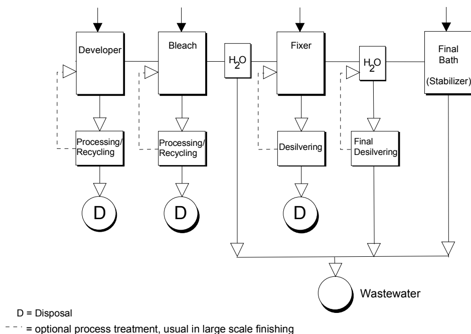
Figure 5 Colour negative film process (C-41)
