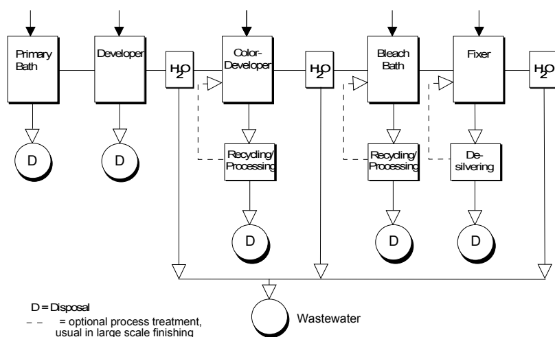
Figure 13 Cine and TV-film reversal process (VNF-1)
