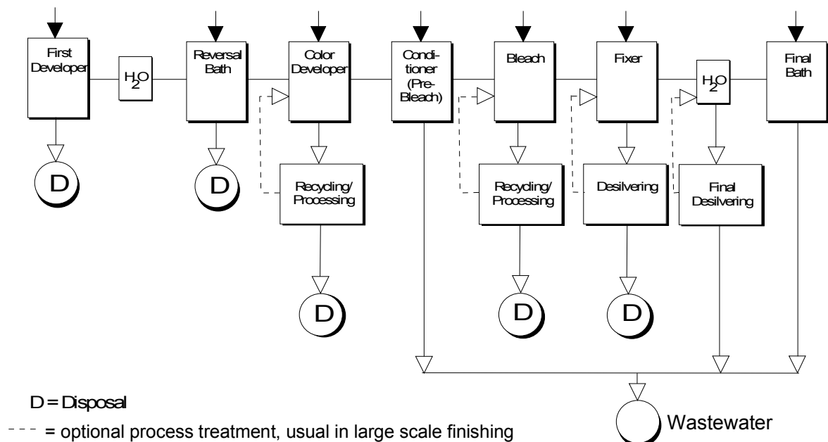
Figure 8 Colour reversal film process (E-6)
