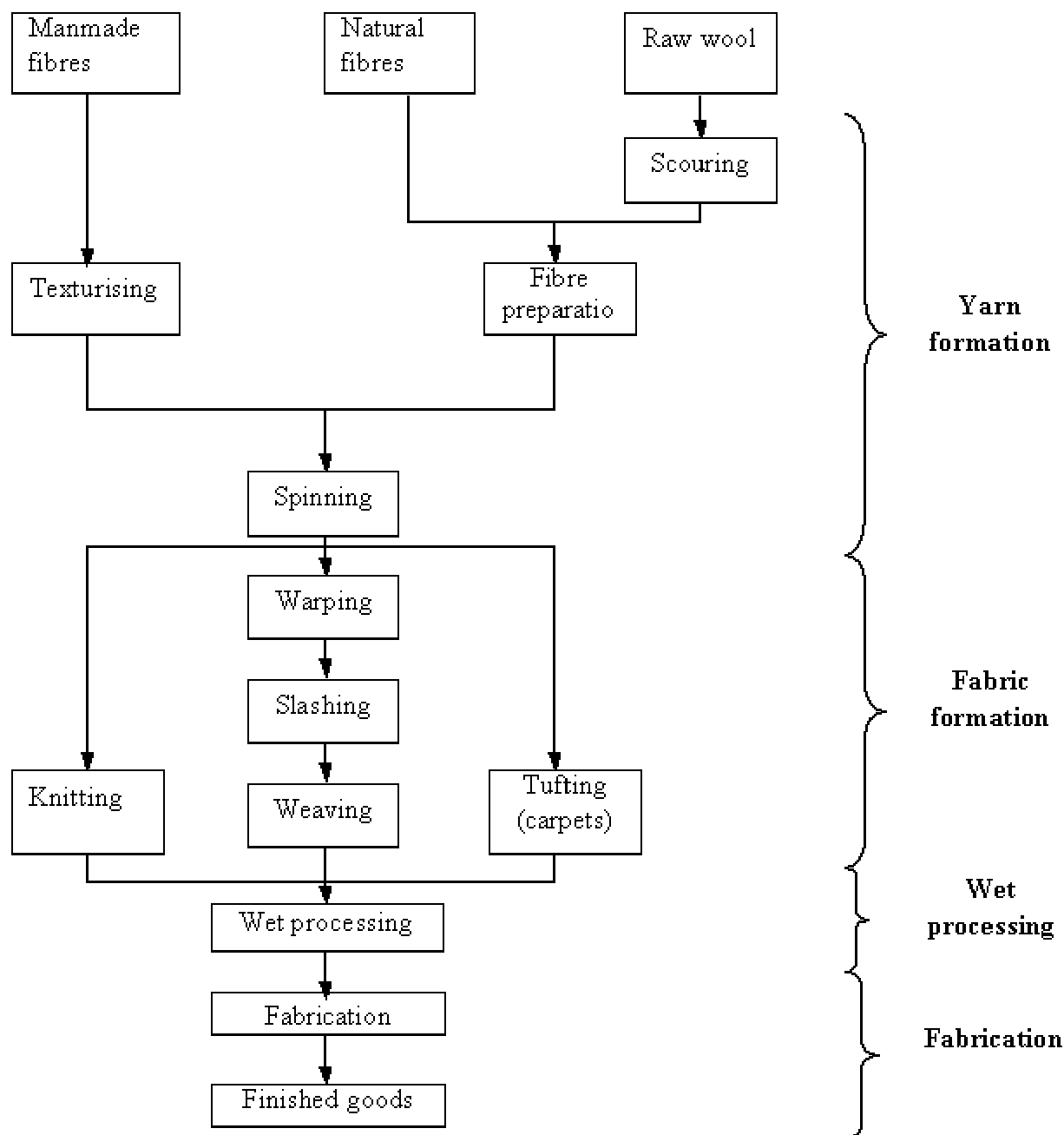
Figure 1 Typical Textile Processing Flow Chart (US EPA, 1997)
